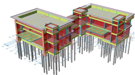
Residential Building Reinforced Concrete Frames Total Area: 615 sq. meters
